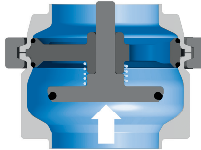
Valve position: Open
